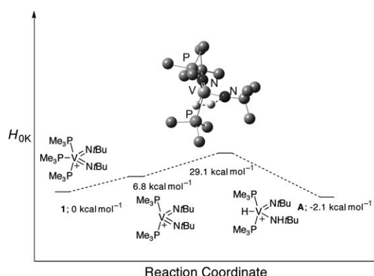
Figure 2. Free enthalpy of \text{H}_2 addition to complex 1 .
