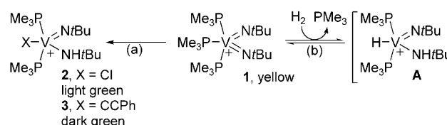
Scheme 1. Conditions: a) 1.05 equiv 2.0 M HCl in \text{Et}_2\text{O} , RT, over night, 46 %; b) 1.05 equiv phenylacetylene in \text{Et}_2\text{O} , RT, 71 %; c) 1 atm \text{H}_2 , \text{PhCF}_3 . In complexes 1 , 2 , 3 , and A the counteranion, [\text{Al}(\text{PFTB})_4]^- , is not depicted for clarity.
